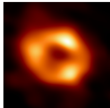
Sagittarius A Image credit: EHT Collaboration
