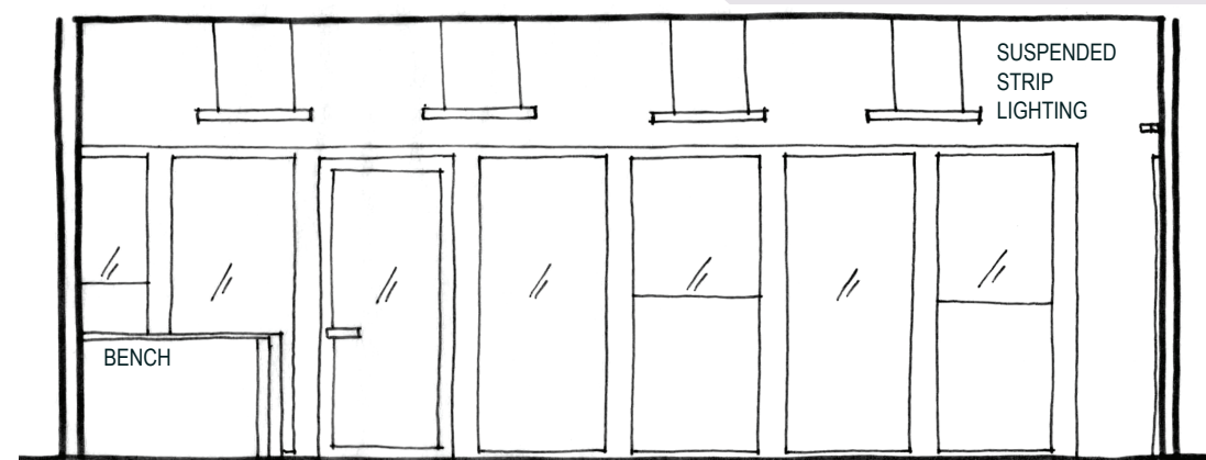
LEARNING SPACE 3 ELEVATION 3
